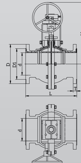
SECTIONAL VIEW
